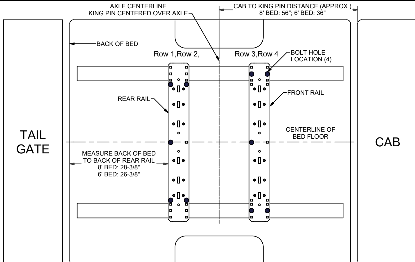
FIGURE 2: RAIL LOCATION DIAGRAM
